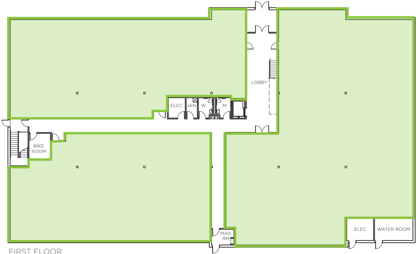
FIRST FLOOR
